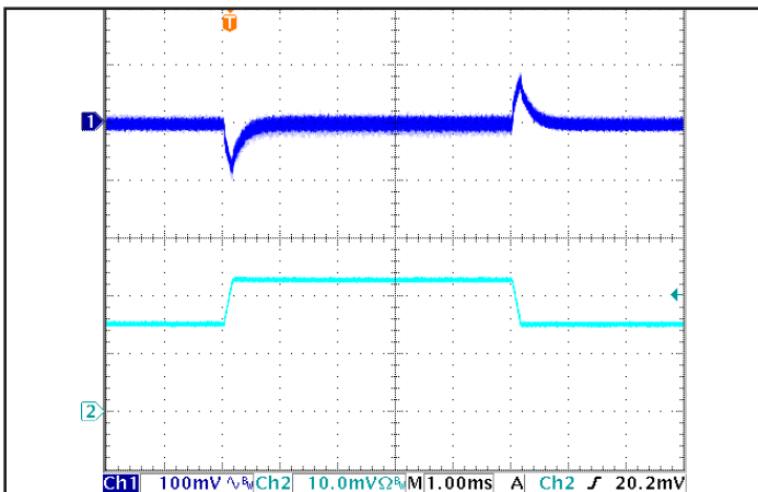
Figure 5: Output voltage response to step-change in load current (50% -75% -50% of Iout(max); dI/dt = 0.1 A/μs). Load cap: 15 μF Tantalum + 1 μF Ceramic capacitor. Ch 1: Vout, Ch 2: Iout (20 A/div).
